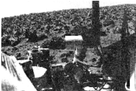
View of the planet Mars from the U.S. Viking mission.
